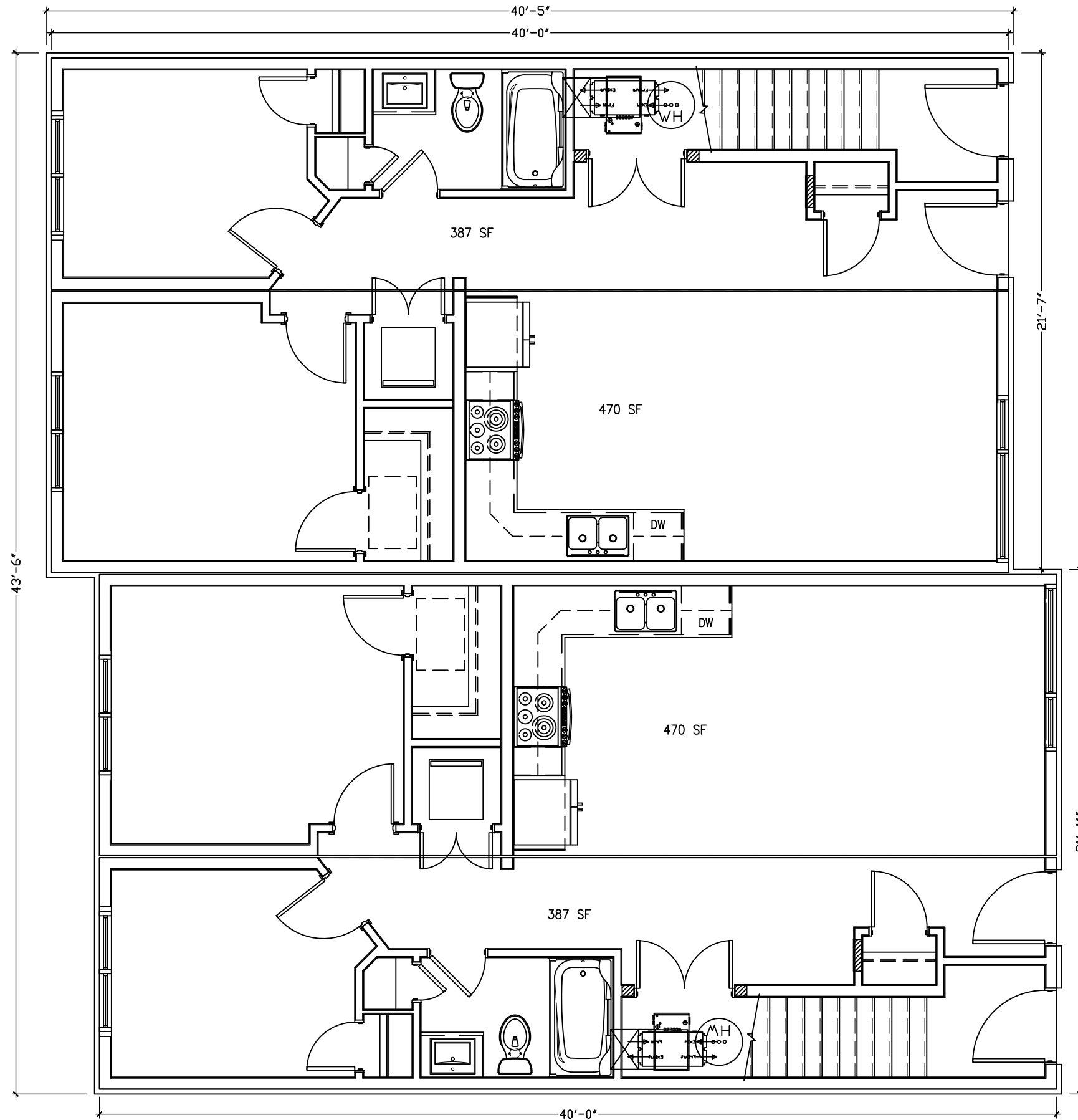
LEVEL 1 FLOORPLAN
